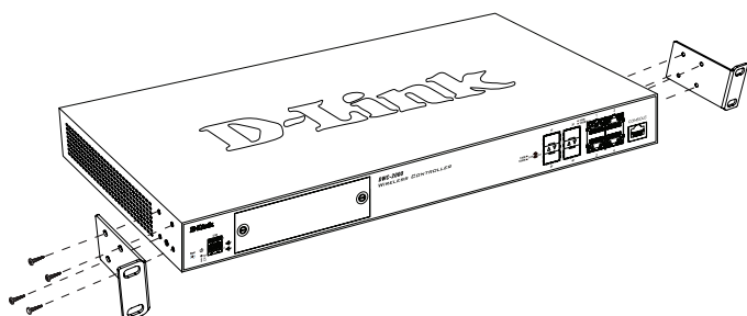
Figure 5. Mounting Brackets
